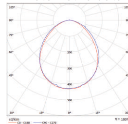
Photometric data
